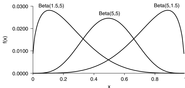
Figure 3.10 Density functions of the Beta(1.5, 5), Beta(5, 5), and Beta(5, 1.5) distributions.
